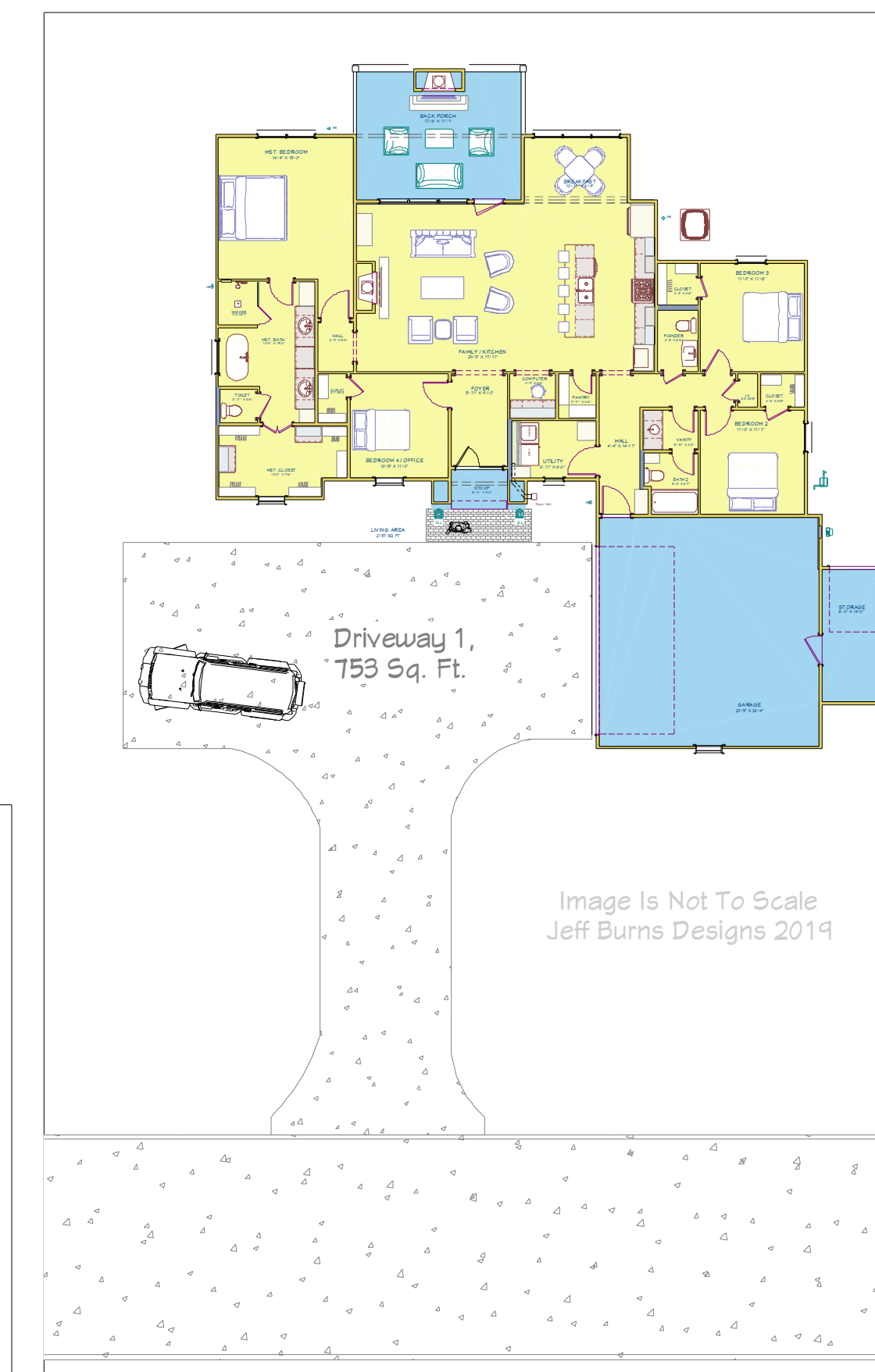
FLOOR PLAN
